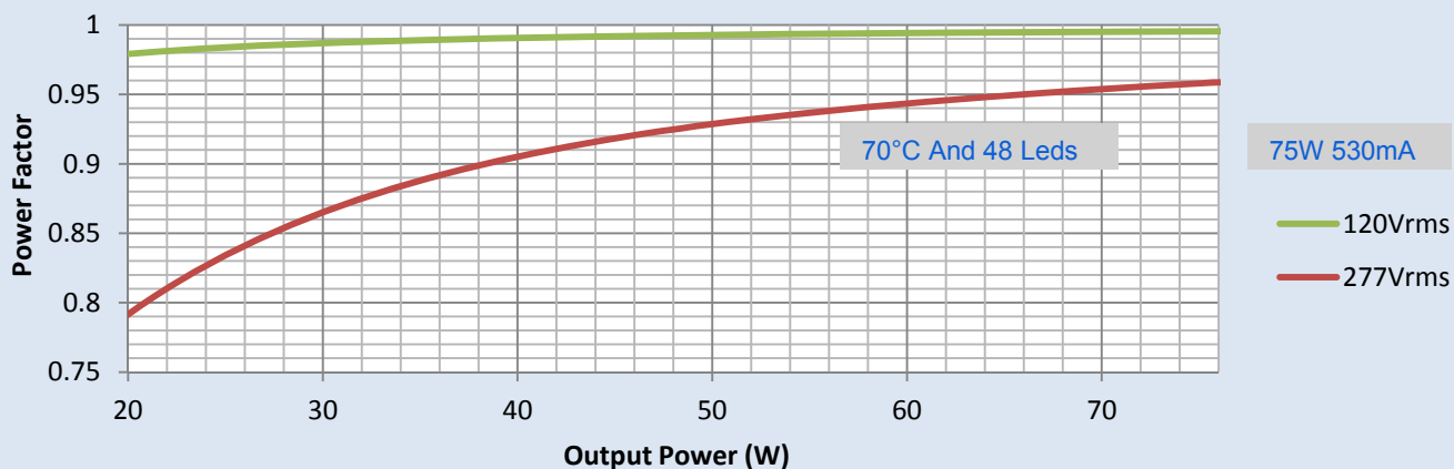
Power Factor Vs. Output Power
