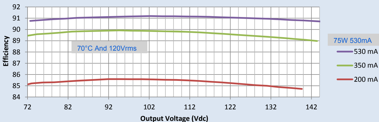
Efficiency Vs. Output Voltage
