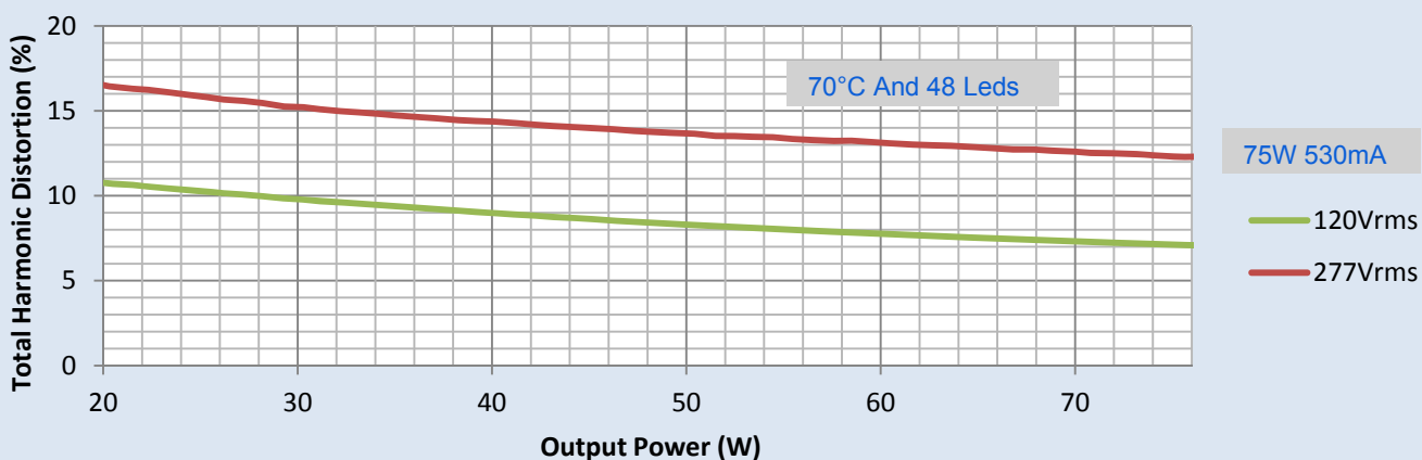
Total Harmonic Distortion Vs. Output Power
